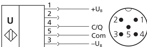
Fig. 3: Connection diagram of the crm+ sensor
