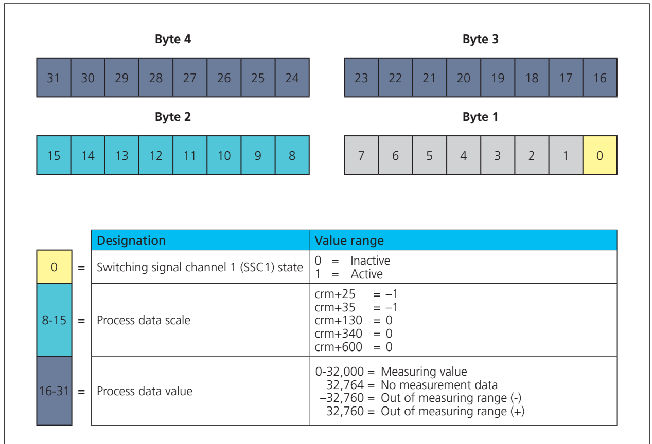
Fig. 4: Process data structure
